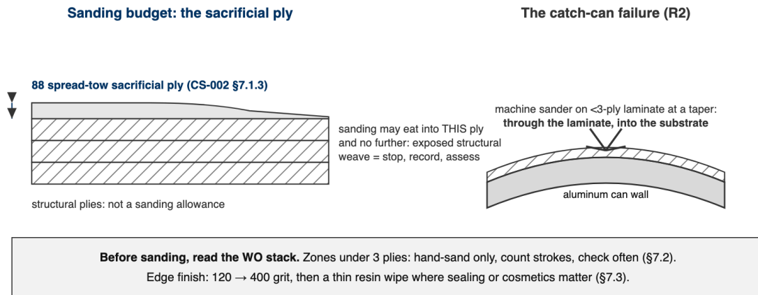
Figure 1: Figure 1. Left: the sacrificial ply is the sanding budget; structural plies are not an allowance. Right: the catch-can failure, a machine sander on thin laminate at a taper, through the skin and into the substrate.
